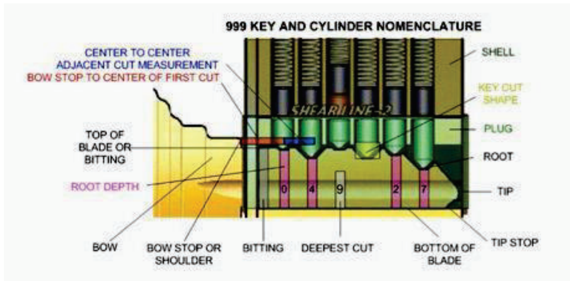
Above: a pin-tumbler lock
